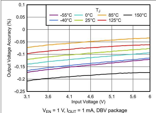
Figure 6-23. Output Voltage Accuracy vs V_{IN}
