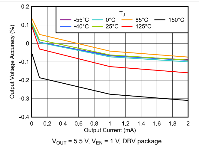
Figure 6-20. Output Voltage Accuracy vs I_{OUT}
