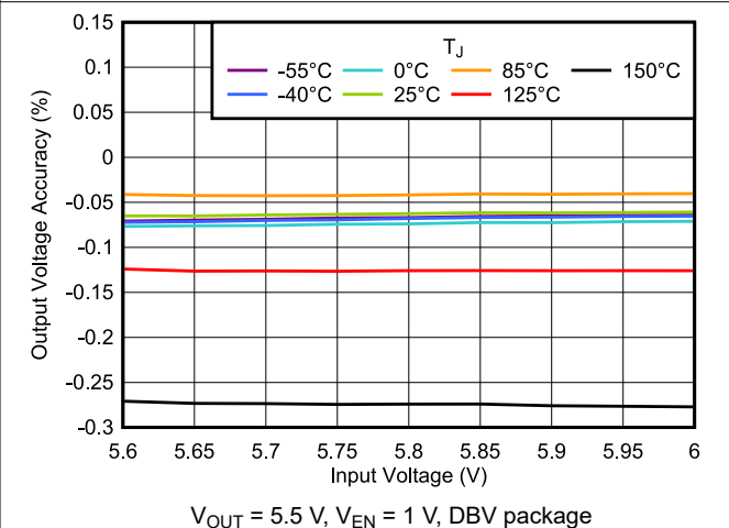
Figure 6-24. Output Voltage Accuracy vs V_{IN}
