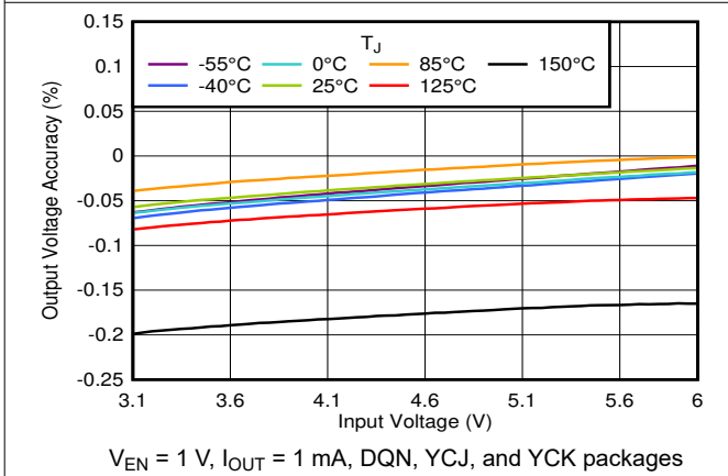
Figure 6-21. Output Voltage Accuracy vs V_{IN}
