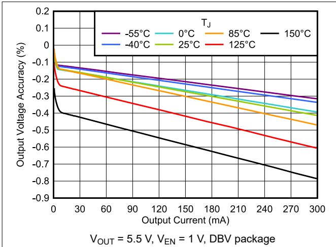
Figure 6-19. Output Voltage Accuracy vs I_{OUT}
