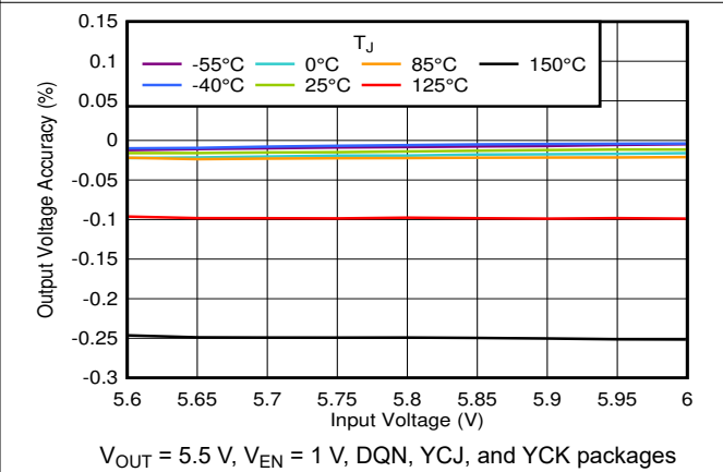
Figure 6-22. Output Voltage Accuracy vs V_{IN}
